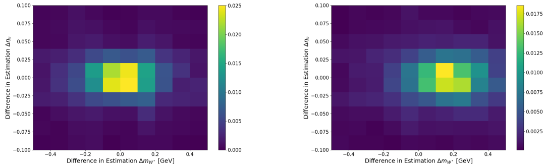
Figure 8.3.: Comparison of two heatmaps showing the difference between the estimated and true values. The two heatmaps use (left) the correct m_H = m_H^{\text{MC}} and (right) the off-set m_H = 125.20 GeV.
