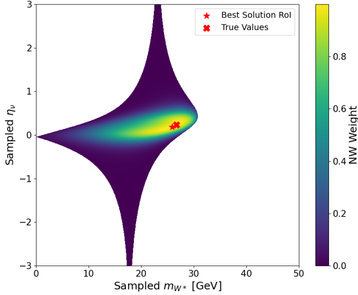
Figure 6.1.: Example of the samples weight distribution for a cherry-picked event. The highest weighted solution (star) and the true values (cross) are marked.
