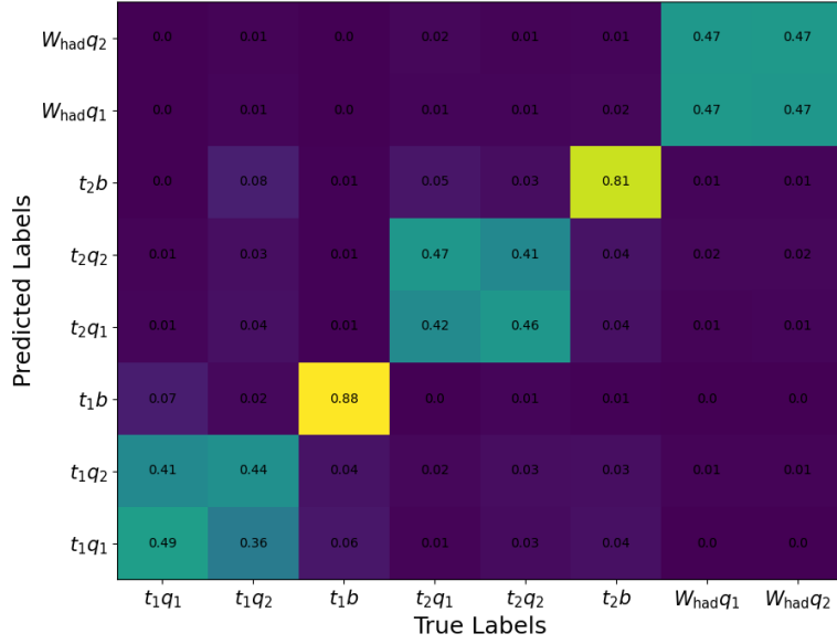
Figure 8.1.: Overview of SPA-Net assignment matrix showing the predicted and true labels. Each column is normalised to unity. Only events with all partons matched are included.
