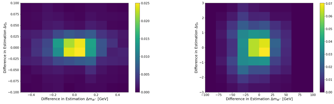
Figure 8.4.: Comparison showing the Neutrino Weighting output difference when using (left) true informatio and (right) reconstructed information as input.
