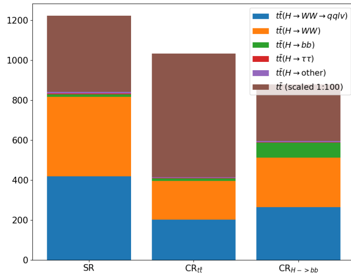
Figure 7.4.: Overview of the region definition. For visual clarity, the t\bar{t} events have been scaled down by a factor of 100.
